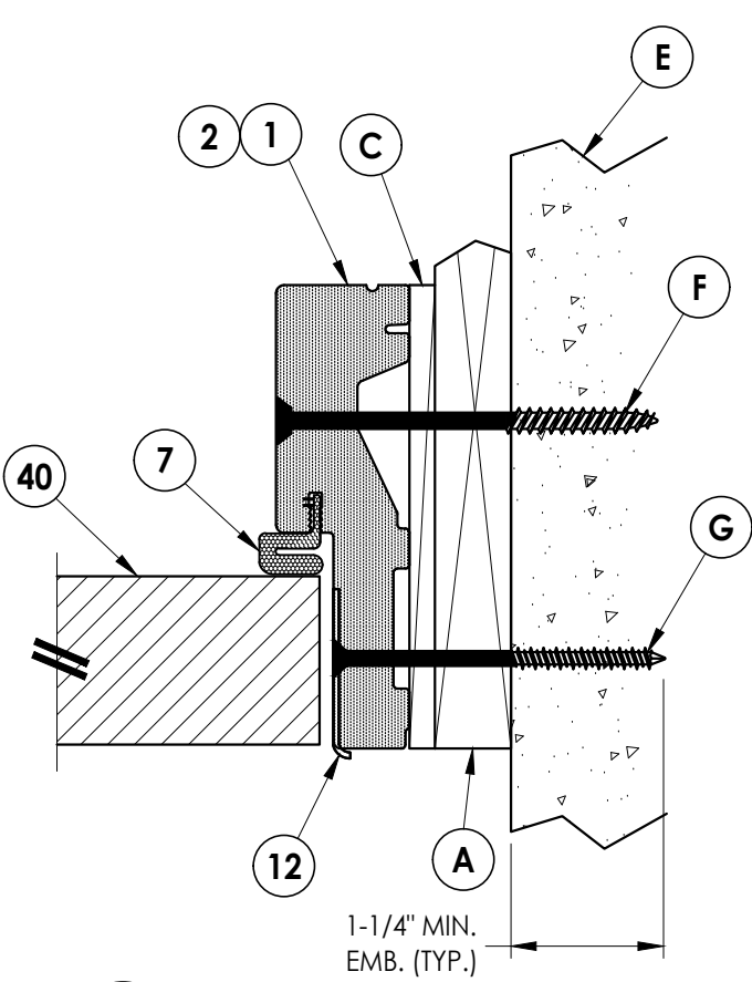
2 7 HORIZONTAL CROSS SECTION Shown w/ 1X sub-buck
