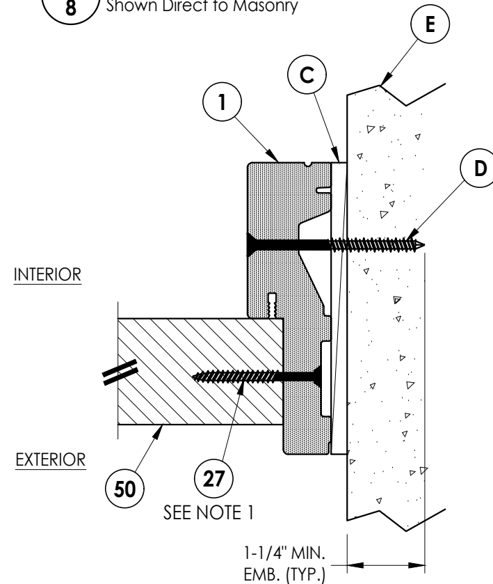
3 HORIZONTAL CROSS SECTION 8 Shown Direct to Masonry
