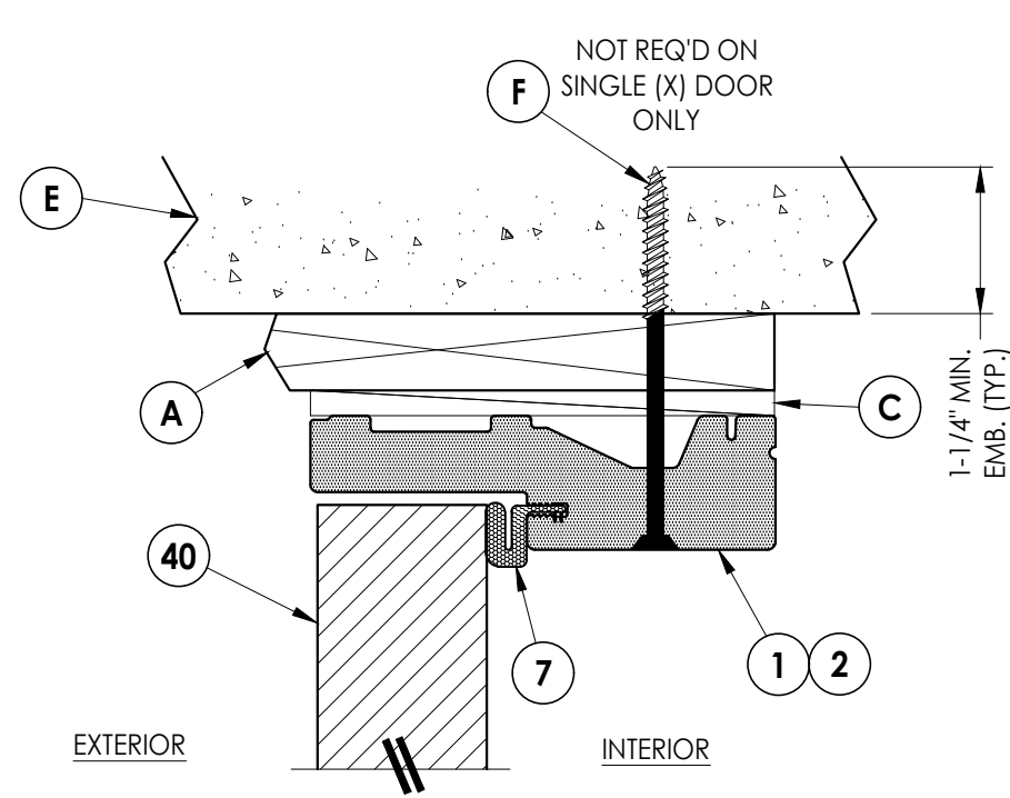
4 7 VERTICAL CROSS SECTION Shown w/ 1X sub-buck
