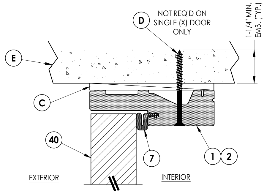
4 VERTICAL CROSS SECTION 8 Shown Direct to Masonry
