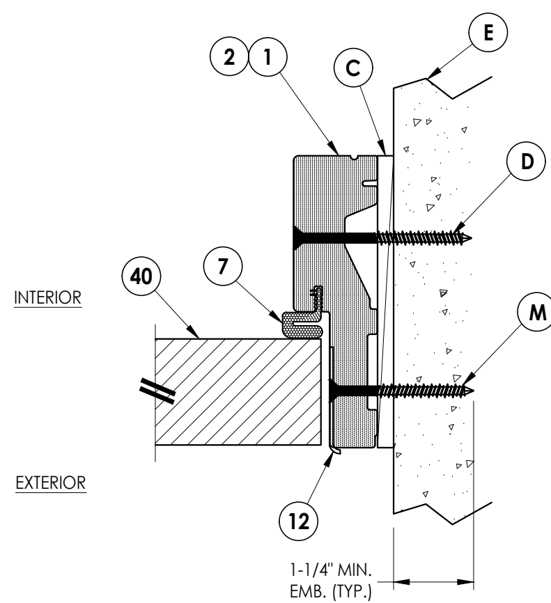
2 HORIZONTAL CROSS SECTION 8 Shown Direct to Masonry
