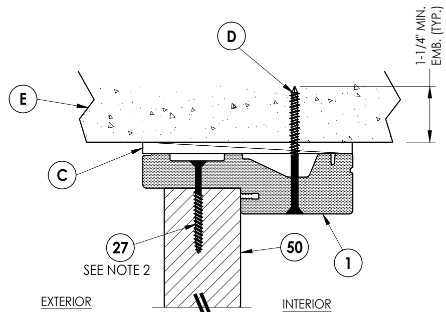
5 VERTICAL CROSS SECTION 8 Shown Direct to Masonry
