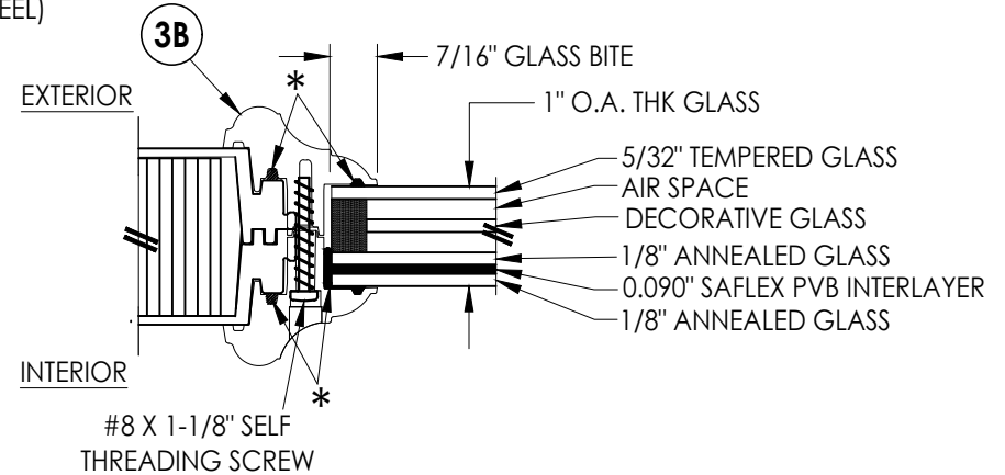
G2 GLAZING DETAIL DECORATIVE GLASS
