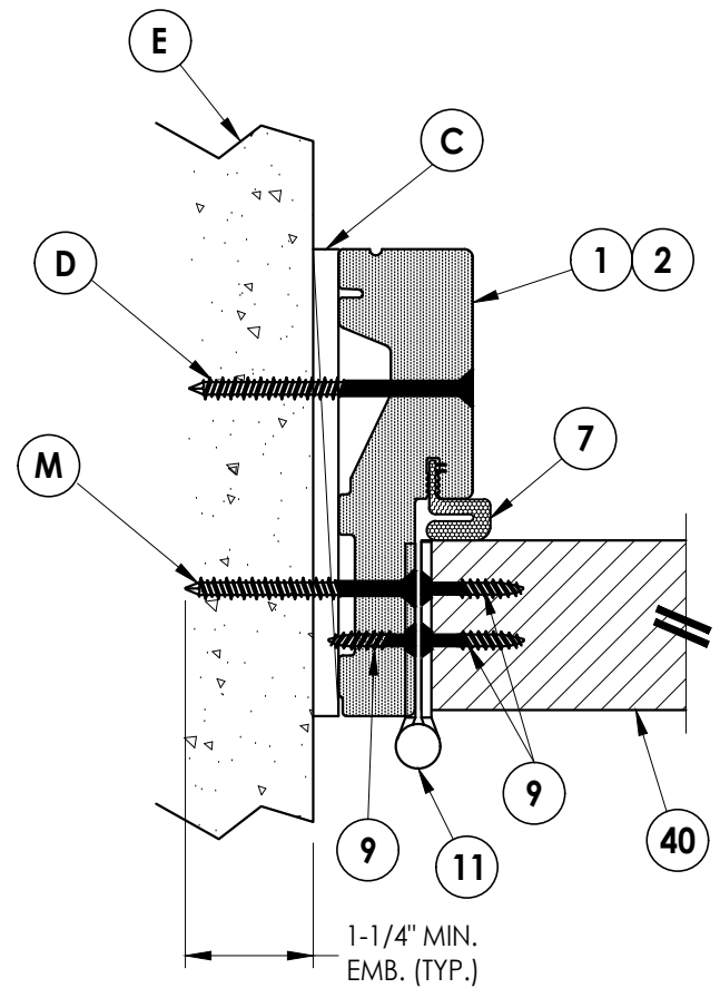
1 HORIZONTAL CROSS SECTION 8 Shown Direct to Masonry
