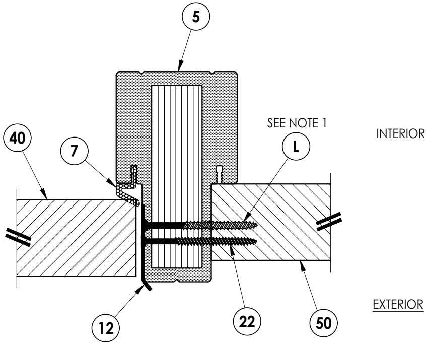
3 5 HORIZONTAL CROSS SECTION SHOWN w/ FAT BOY MULLION
