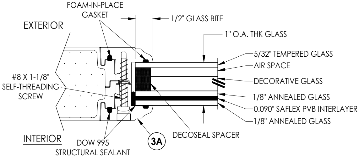
G2 GLAZING DETAIL Triple Pane
