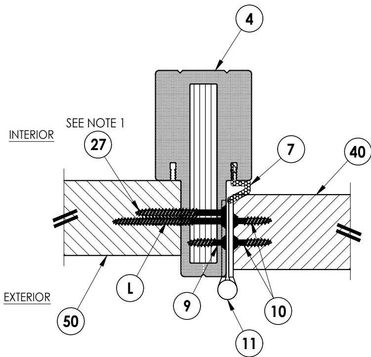
1 5 HORIZONTAL CROSS SECTION Outswing Shown (Inswing Similar)
