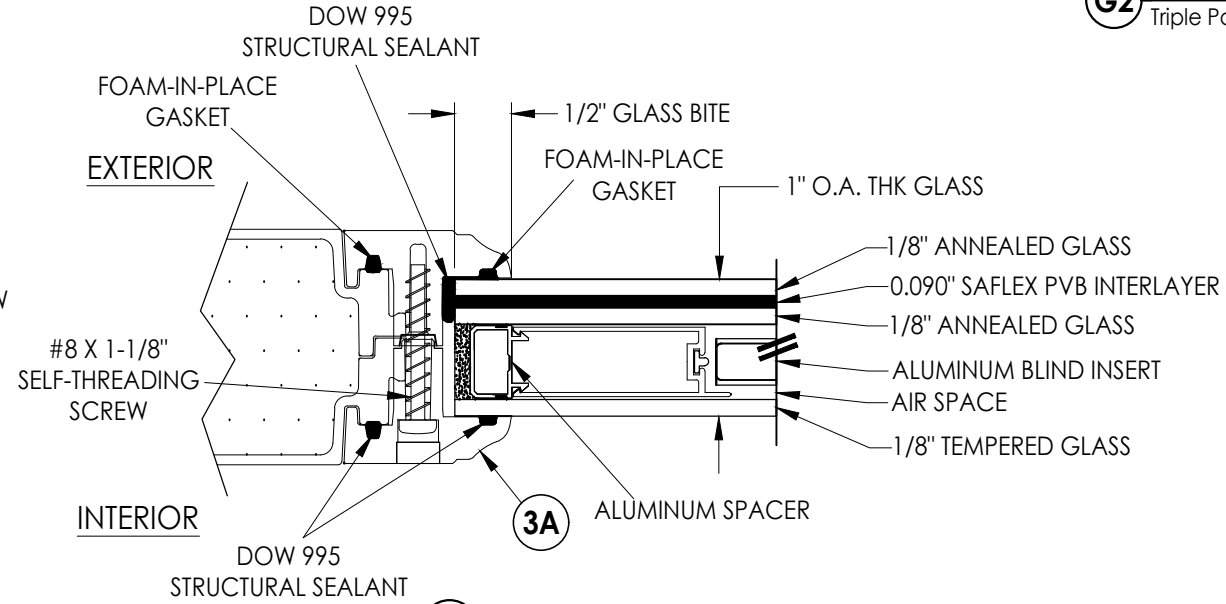
G3 GLAZING DETAIL Blinds Between Glass
