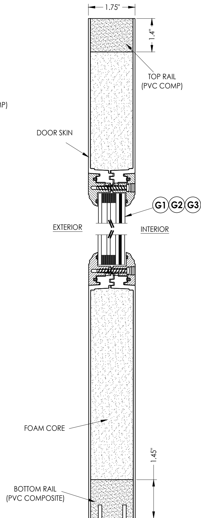
2 VERTICAL CROSS SECTION
