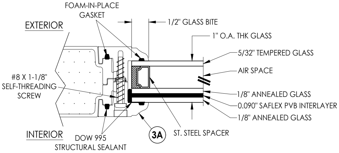
G1 GLAZING DETAIL Dual Pane
