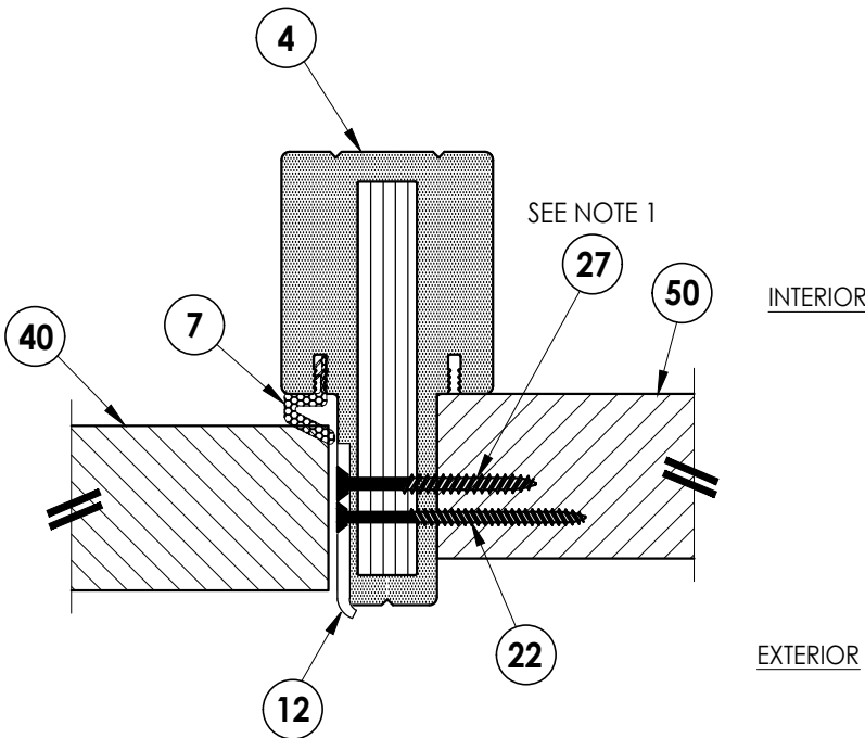
2 5 HORIZONTAL CROSS SECTION Outswing Shown (Inswing Similar)
