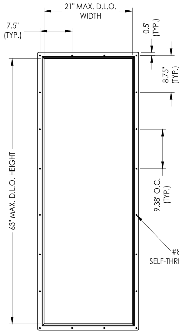
6"-8" LITE FRAME ABS
