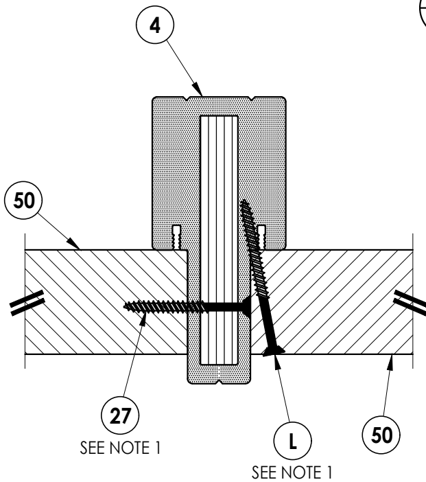
3 5 HORIZONTAL CROSS SECTION Outswing Shown (Inswing Similar)
