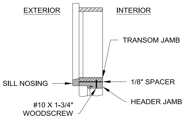
Fig. 2c (Outswing System)
