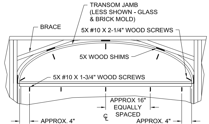
Fig. 2d (Half-round or Elliptical Transom)
